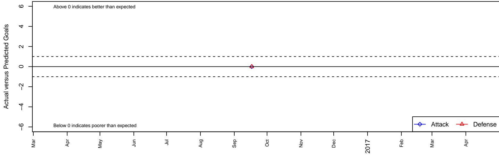
Central Valley SJ Quakes Academy G03 Dots are actual minus expected GF (blue circles) and GA (red triangles). Blue line is smoothed change in attack strength. Red is smoothed change in defense strength.
